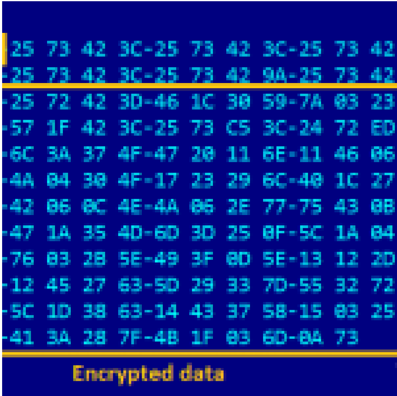
Figure 8. Data sent by the C&C
